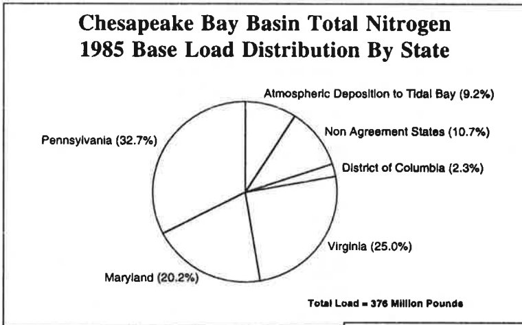
Figure 4a. Chesapeake Bay Basin Total Nitrogen 1985 Base Load Distribution By State (Source: 1991 Watershed Model)
