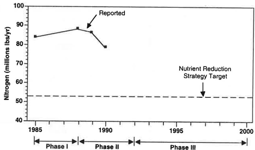
Figure 6a. Point Source Nitrogen Reduction Progress (Source: see references 7, 8)
