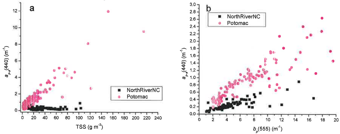
Figure 13. Comparison of NAP absorption for the Potomac River with that of the North River, North Carolina. a) Non-algal particulate absorption at 440 nm versus total suspended solids (TSS). b) Non-algal particulate absorption at 440 nm versus scattering coefficient at 555 nm. Slopes of the relationships indicate that particle color index (PCI), i.e. the ratio of non-algal particulate absorption at 440 nm to particulate scattering at 555 nm, is less variable than specific-absorption coefficients. Data in (b) were truncated to facilitate comparison.
