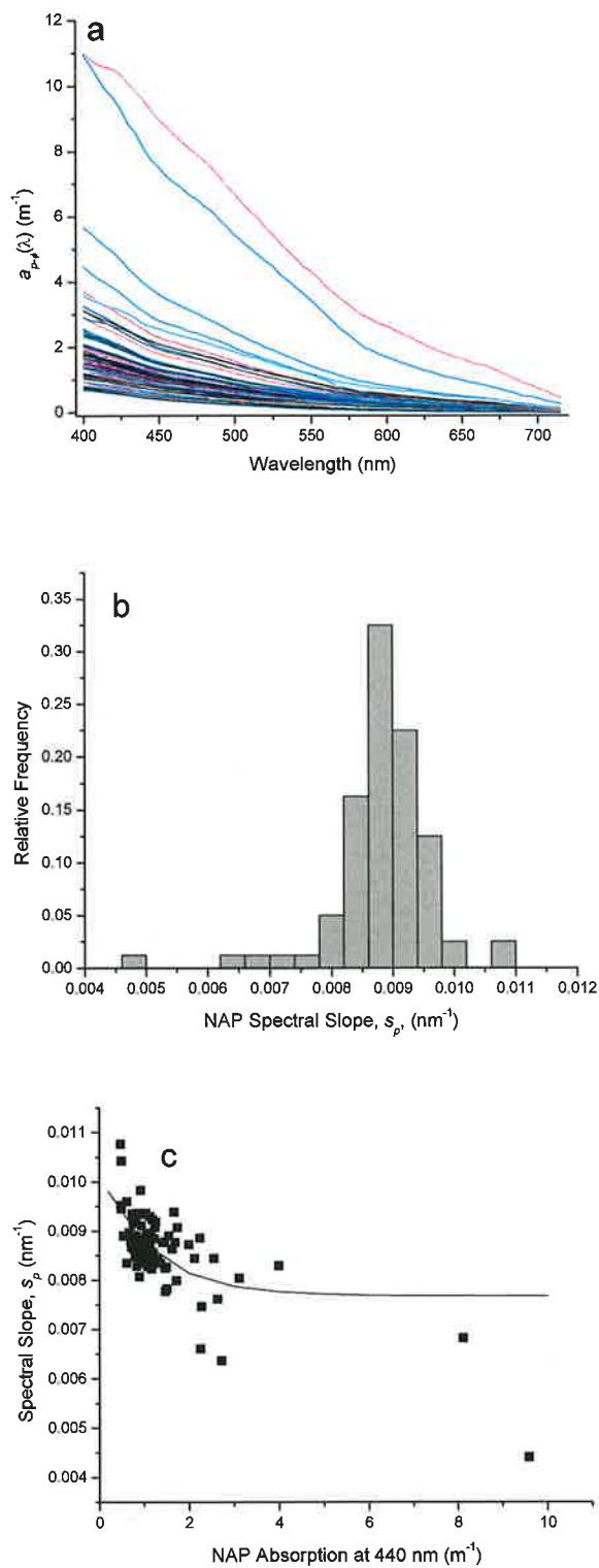
Figure 8. Absorption by non-algal particulates (NAP). a) Non-algal particulate absorption spectra. b) Histogram of NAP spectral slopes. c) Spectral slope versus NAP absorption at 440 nm. Solid line is calculated by equation 32.
