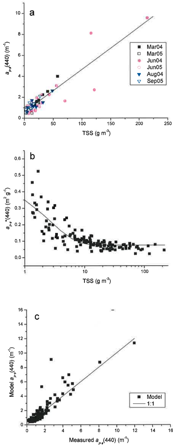
Figure 9. Relationship of non-algal particulate (NAP) absorption to total suspended solids (TSS). a) Linear relationship between NAP absorption at 440 nm and TSS. Like symbols represent the same season. b) Specific-absorption coefficient of NAP calculated on a sample-by-sample basis versus TSS. Solid line is calculated by equation 33a. c) Modeled (equation 33b) versus measured NAP absorption at 440 nm. See text for further discussion.
