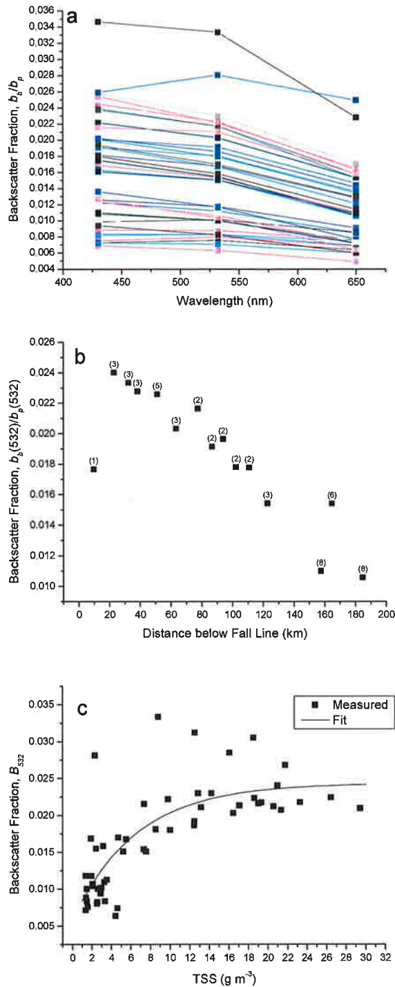
Figure 12. Backscattering. a) Backscatter fraction for 43 profiles within instrument range. b) Backscatter fraction for 62 measurements of the green (532 nm) sensor versus river kilometer. The numbers above the points are the number of observations available per station. c) Relationship between the backscatter fraction at 532 nm and total suspended solids (TSS). The solid line is estimated by empirical fit (equation 35).
