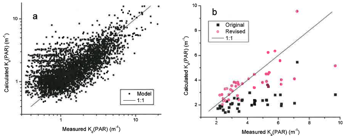
Figure 16. a) Diffuse attenuation coefficients for PAR calculated by the lookup table approach plotted against measured values from the Chesapeake Bay Water Quality Monitoring Program, 1995-1999; 1:1 line is provided for reference. b) Diffuse attenuation coefficients for PAR calculated by the lookup table approach plotted against measured values for oligohaline Mataponi River (MPNOH) with (black squares) originally estimated values for specific-scattering coefficient and particle color index, and (red circles) adjusted parameters determined using an inverse solution on median measured K_d(\text{PAR}) and water quality concentrations.
