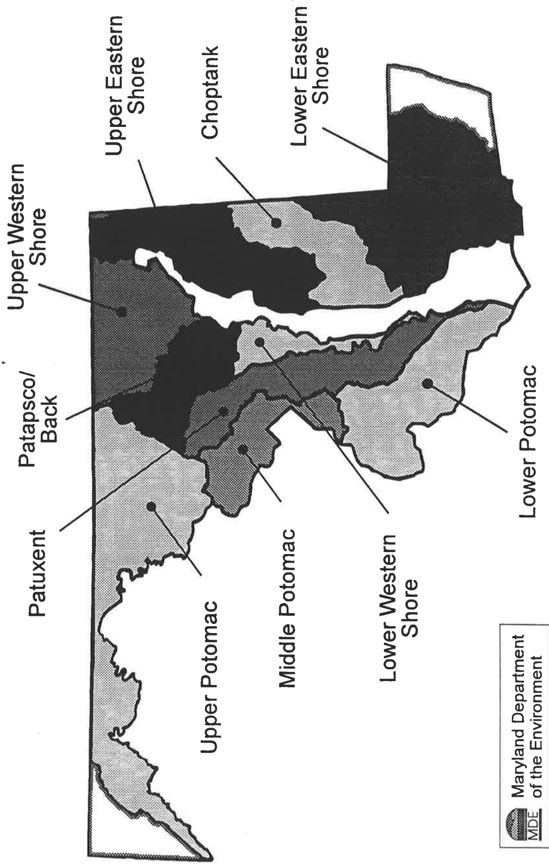
Figure 1. Maryland's Tributary Watersheds
