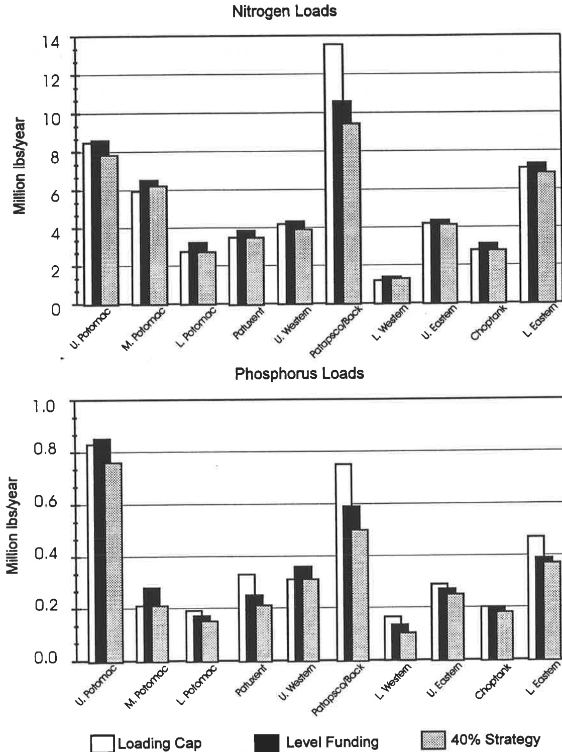
Figure 2. Level Funding and 40% Strategy Projected Nutrient Loadings
