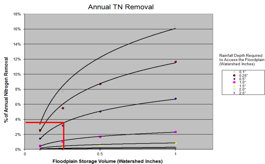
Figure 67. Annual TN removal as a function of 0.25 watershed inch 3 floodplain storage volume and 0.5 inch rainfall depth required to access the floodplain.
