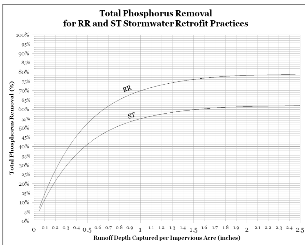
Figure 6. Percent phosphorus removal for runoff reduction and stormwater treatment (Schueler and Lane 2012a). Note: RR = runoff reduction BMPs and ST= stormwater treatment BMPs
