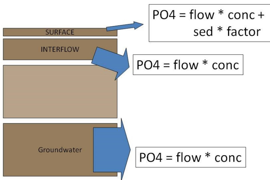
Figure 3. Representation of how P export is simulated in PQUAL module of the CBWM (Source: Presentation to Expert Panel by Matt Johnston, CBPO, February 19, 2013).
