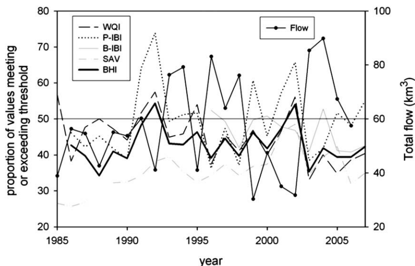
Fig. 3. Time series of the Water Quality Index (WQI), Phytoplankton Index of Biotic Integrity (P-I-BI), Benthic Index of Biotic Integrity (B-I-BI), Submerged Aquatic Vegetation (SAV), the Bay Health Index (BHI) and total flow to the Chesapeake Bay (1985–2007). Not including flow, values are area-weighted means of the proportion of values meeting or exceeding assessment thresholds for each of the 15 reporting regions. Note that Bay-wide B-I-BI data were first available in 1996.
