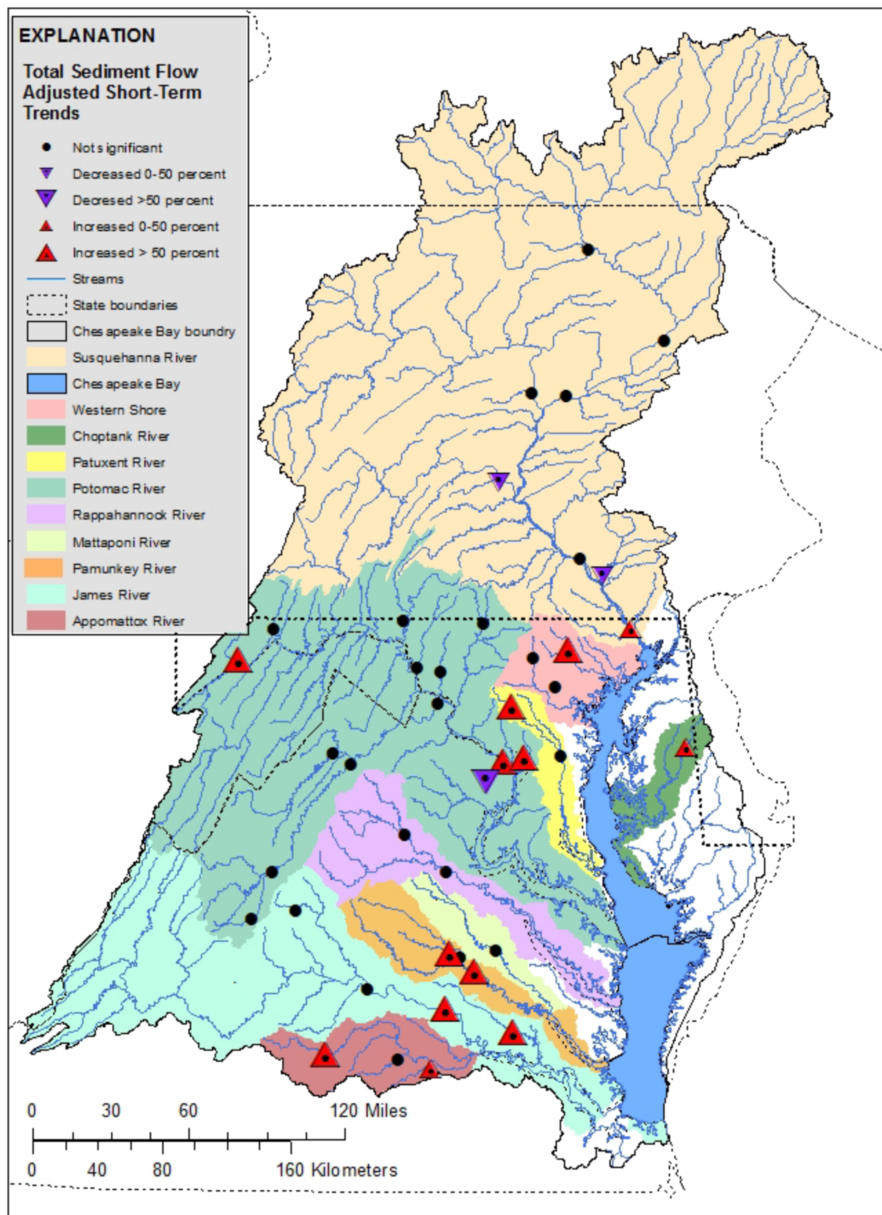
Flow-adjusted trends for total sediment for 41 sites in the Chesapeake Bay Watershed, 2002-2011.
