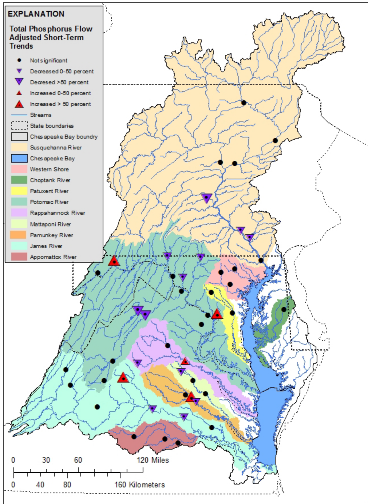
Flow-adjusted trends for total phosphorus for 47 sites in the Chesapeake Bay Watershed, 2002-2011.
