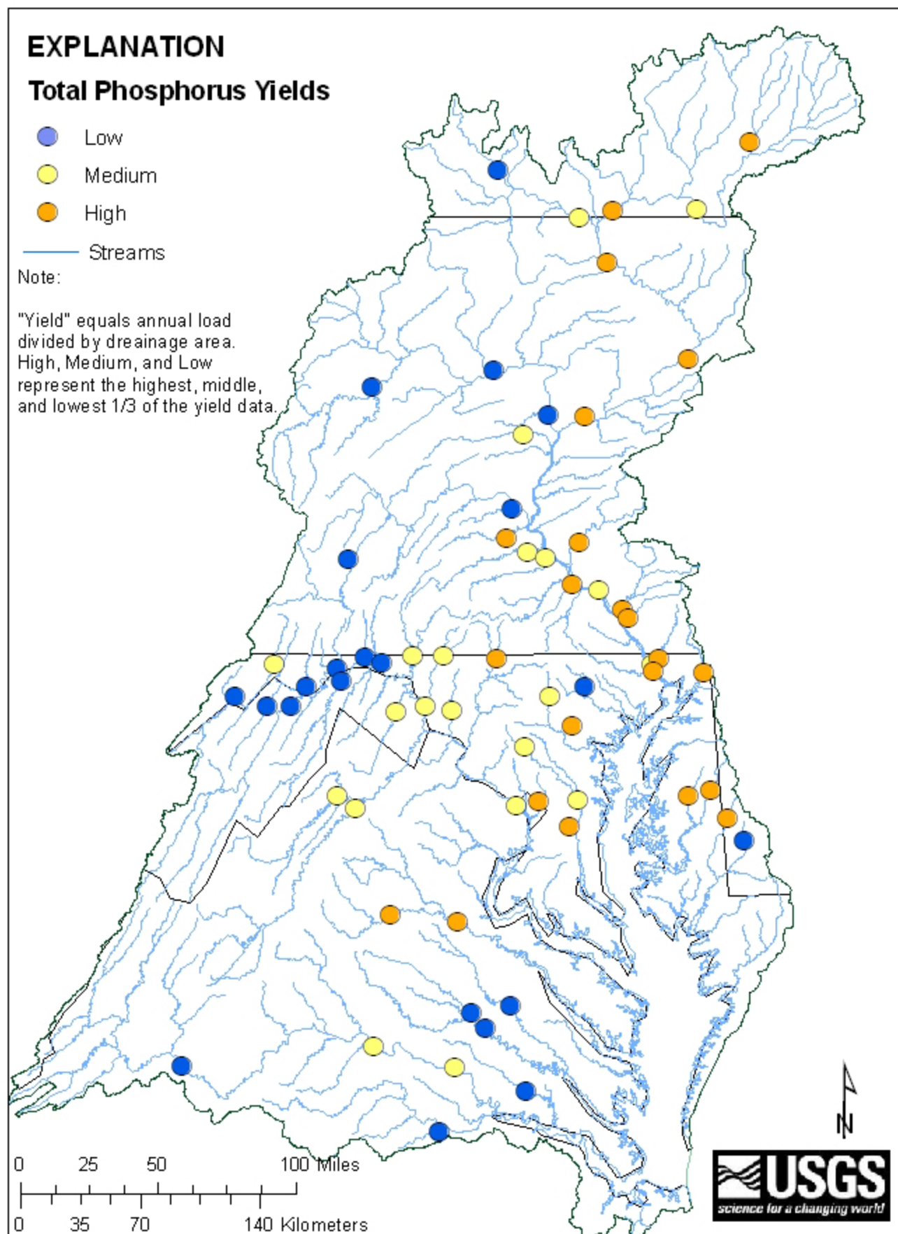
Total phosphorus yield for 65 sites in the Chesapeake Bay Watershed.
